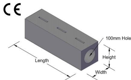
10" x 10" Slotted Drainage Channel
